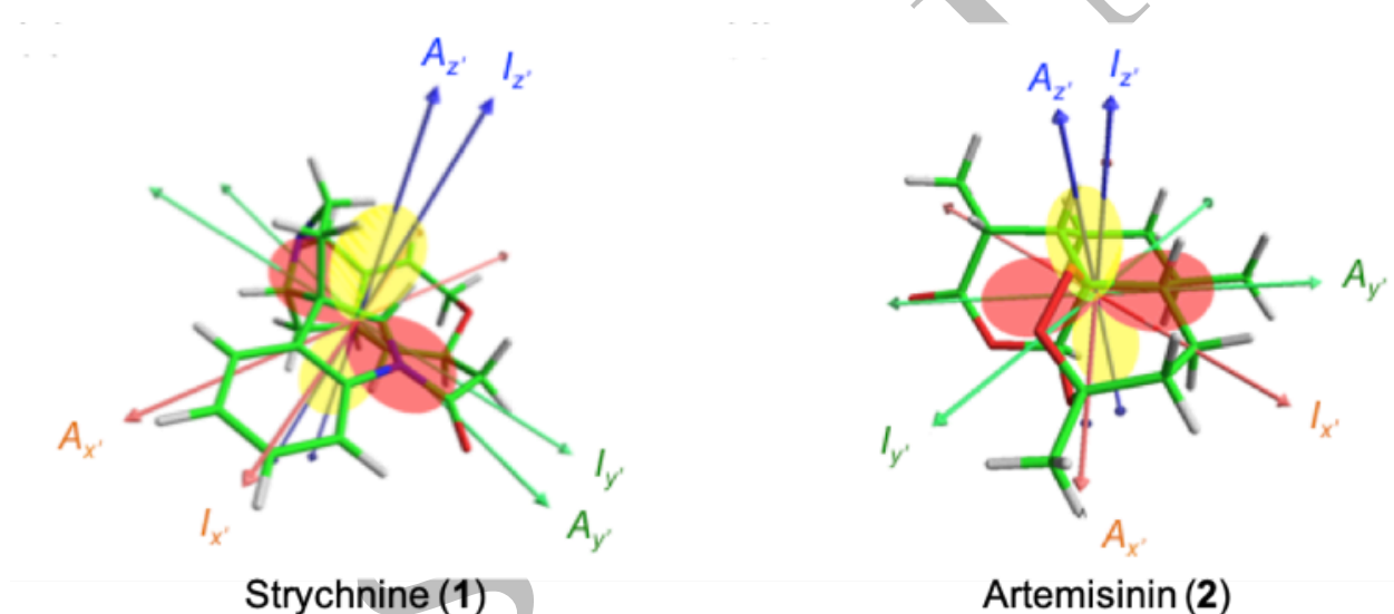
Figure 3. Displaying of principal axis system ( A_{x'} , A_{y'} , A_{z'} ) of the diagonalized alignment tensor, the inertia tensor axes, ( I_{x'} , I_{y'} , I_{z'} ) and the Saupre tensor surface representation (pink and yellow surfaces indicate positive and negative ^2\text{H-RQCs} , respectively) of 1 and 2 oriented in PBLG/ \text{CHCl}_3 .
