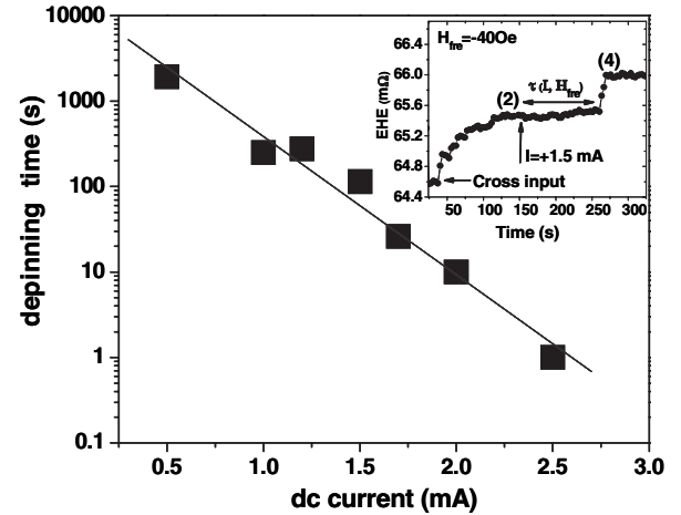
FIG. 4. Depinning time \tau(I, H_{\text{fre}}) at position (2) as a function of dc current for H_{\text{fre}} = -40 Oe. Inset: typical measurement of \tau(I, H_{\text{fre}}) for a DW initially at the cross input. Under H_{\text{fre}} = -40 Oe, the DW propagates by discrete jumps of about 10 nm until it remains pinned at position (2) [cf. Fig. 1(d)]. Then a dc current I is applied (in this case, +1.5 mA) and the depinning time, \tau(I, H_{\text{fre}}) , is measured.
