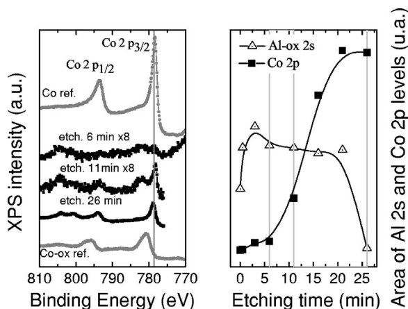
FIG. 3. (a) Co 2p XPS spectra corresponding to an oxidation of 90 s recorded after different etching times. The gray plots are Co and Co oxide reference spectra. (b) Area of Al oxide 2s and Co 2p levels vs etching time. Each vertical gray line corresponds to an etching time after which XPS spectra presented in (a) are recorded.
