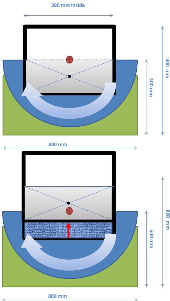
Figure 4: The axis of rotation (fixed) may be relatively more (top) or less (bottom) elevated than the cargo's center of gravity. The red arrow represents 112.5mm maximum.
