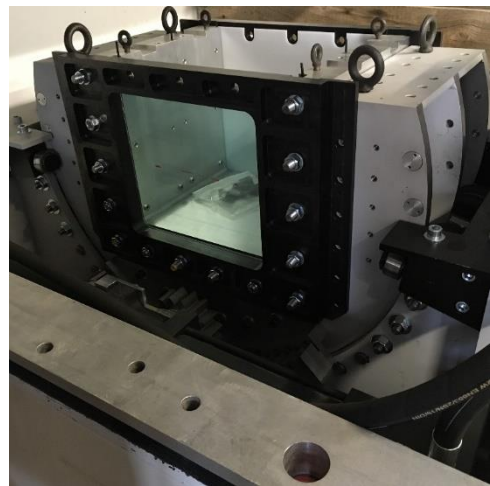
Figure 3 : Detail of the IFSTTAR's Rolling box
