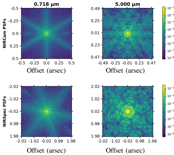
Fig. 3. PSFs of the NIRCam Imager (top) and NIRSpec IFU (bottom) calculated with webbpsf [42] for two particular wavelengths (logarithmic scale).
