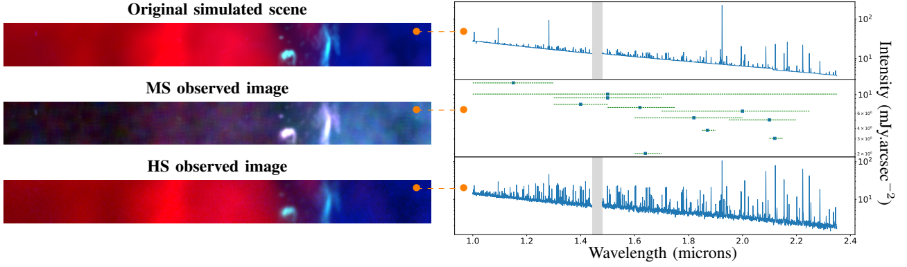
Fig. 2. Left: RGB compositions of the synthetic simulated scene (top), the NIRCam Imager MS image (middle) and the NIRSpec IFU HS image (bottom) [Red channel: \text{H}_2 emission line pic intensity at 2.122\mu\text{m} , Green channel: \text{H} recombination line pic intensity at 1.865\mu\text{m} , Blue channel: \text{Fe}^+ emission line pic intensity at 1.644\mu\text{m} ]. Right: A spectrum from 1.0 to 2.35 microns related to a pixel of each image on their left. From top to bottom, the first two are original spectra from the synthetic scene with 4974 points, the following two are observed spectra from the multiband image provided by the NIRCam Imager forward model with 11 spectral points, the last two are calibrated observed spectra from the HS image provided by the NIRSpec IFU forward model with about 5000 spectral points.
