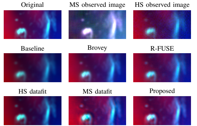
Fig. 5. Zooms on strong structures excerpt from Fig. 2 (simulated, MS observed and HS observed images) and from Fig. 4 (fused images by the compared methods).
