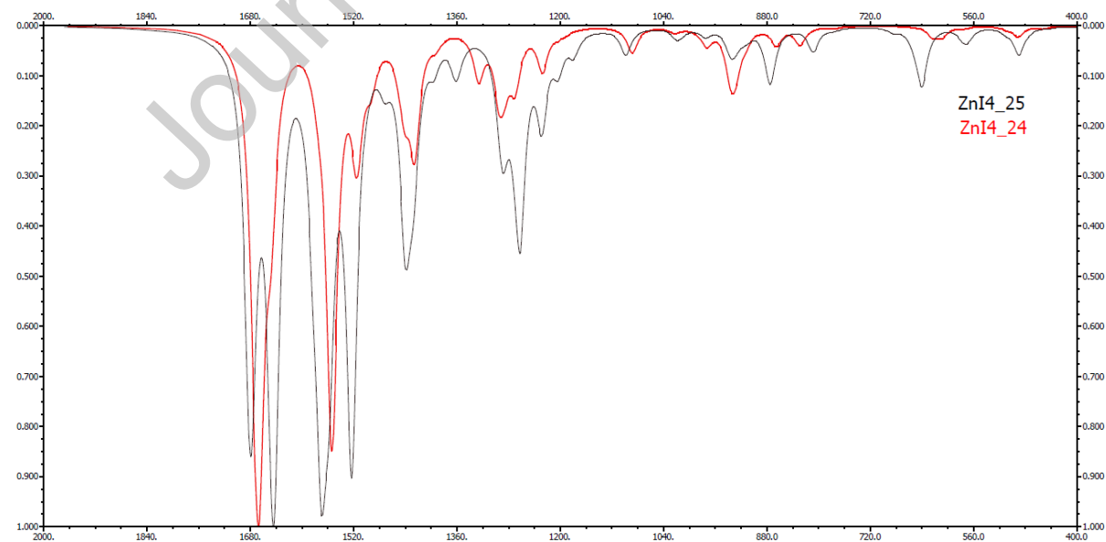
Figure 3: Calculated IR spectra of complex 1 (black) and complex 2 (red) (2000-400 \text{cm}^{-1} )
