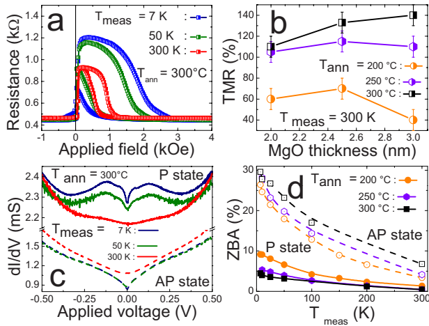
FIG. 1. (Color online) (a) Resistance vs applied field measured at different temperatures ( T_{\text{meas}} ) on a MTJ ( t_{\text{MgO}}=2 nm, T_{\text{ann}}=300 °C); (b) TMR vs t_{\text{MgO}} measured on MTJ at 300 K for three different values of T_{\text{ann}} . Error bars were evaluated from the measure on more than ten different junctions. (c) Differential conductances measured at different values of T_{\text{meas}} on a MTJ ( t_{\text{MgO}}=2 nm, T_{\text{ann}}=300 °C) in the P (continuous lines) and AP (dashed lines) states. (d) ZBA vs T_{\text{meas}} measured on MTJs ( t_{\text{MgO}}=2 nm) measured in the P (continuous lines) and AP (dashed lines) states for three different values of T_{\text{ann}} .
