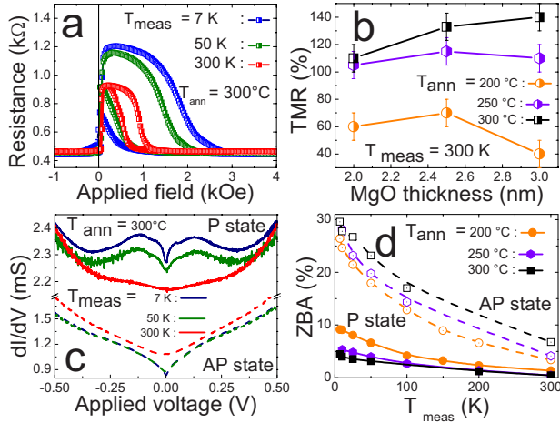
FIG. 1. (Color online) (a) Resistance vs applied field measured at different temperatures ( T_{\text{meas}} ) on a MTJ ( t_{\text{MgO}}=2\text{ nm} , T_{\text{ann}}=300^\circ\text{C} ); (b) TMR vs t_{\text{MgO}} measured on MTJ at 300 K for three different values of T_{\text{ann}} . Error bars were evaluated from the measure on more than ten different junctions. (c) Differential conductances measured at different values of T_{\text{meas}} on a MTJ ( t_{\text{MgO}}=2\text{ nm} , T_{\text{ann}}=300^\circ\text{C} ) in the P (continuous lines) and AP (dashed lines) states. (d) ZBA vs T_{\text{meas}} measured on MTJs ( t_{\text{MgO}}=2\text{ nm} ) measured in the P (continuous lines) and AP (dashed lines) states for three different values of T_{\text{ann}} .
