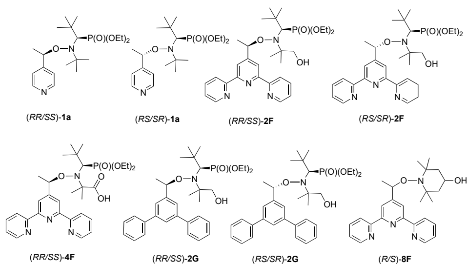
Figure 2. Structures of alkoxyamines 1a , 2F , 4F , 2G and 8F .
