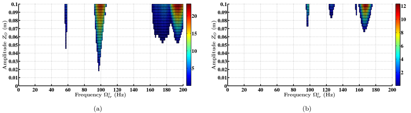
Fig. 21. Stability charts of the rotor excited by sinusoidal translations of the support along the yaw axis and by a mass unbalance ( m_{mu1}r_{mu1} = m_{mu2}r_{mu2} = 6300 g mm) of phases: (a) \eta_{mu1} = \eta_{mu2} = 0^\circ , (b) \eta_{mu1} = 0^\circ , \eta_{mu2} = 180^\circ .
