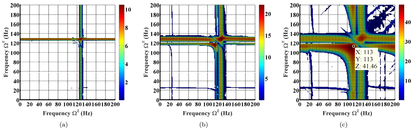
Fig. 15. Stability charts of the rotor excited by combined sinusoidal rotations of the support around the pitch and yaw axes: \beta = \beta^a \cos \Omega^x t and \alpha = \alpha^a \cos \Omega^z t with \beta^a = \alpha^a = (a) 0.05 rad, (b) 0.1 rad, (c) 0.2 rad.
