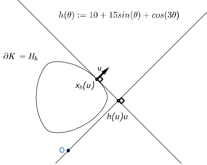
Figure 1. Envelope parametrized by its Gauss map
