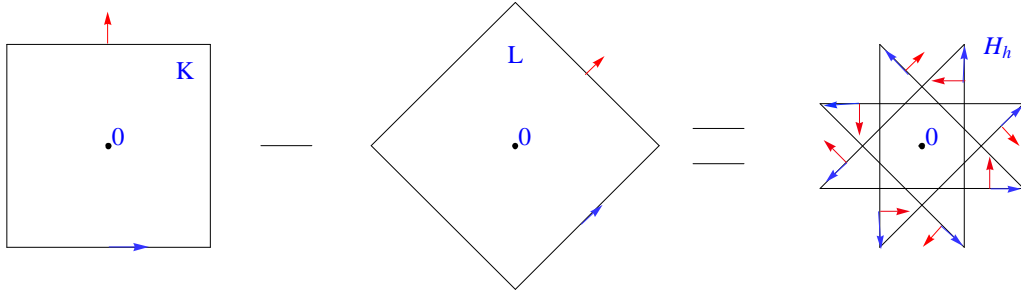
Figure 3. Octagram obtained as the difference of two squares
