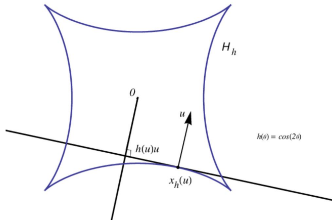
Figure 2. Plane hedgehog with C^2 -support function
