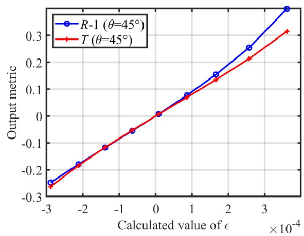
Fig. 4. Comparison of R(\epsilon) and T(\epsilon) for the MILO architecture of [13] ( \theta \approx 45^\circ , Q \approx 15000 , f_0 \approx 68\text{kHz} , V_{bias} \approx 40\text{V} , V_{drv} \approx 450\text{mV} ).
