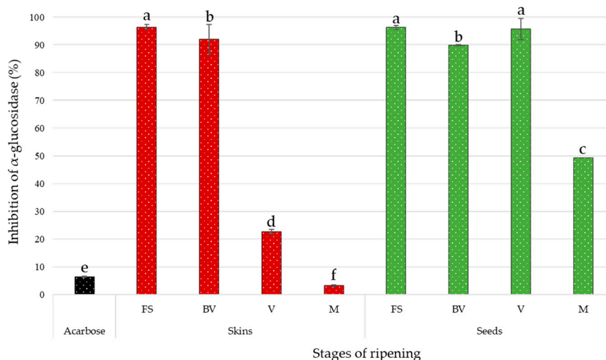
Figure 2. Inhibitory effects of Tannat skin and seed extracts (0.4 g/L) and positive control (acarbose at 0.4 g/L) on \alpha -glucosidase (pH 6.8, T = 37 °C) at different stages of ripening: First Stage (FS), Before Veraison (BV), Veraison (V) and Maturity (M). Values are means of four replicates. Significant differences between treatments at p < 0.05 are indicated with letters as measured by Tukey test.
