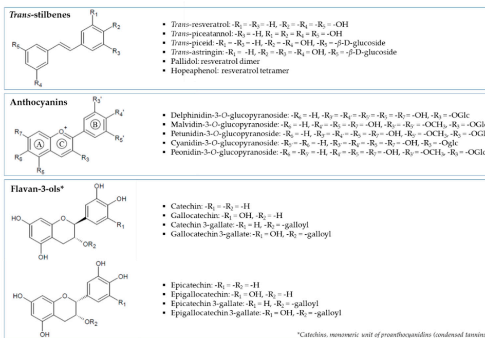
Figure 1. Structures of different polyphenol families and relative compounds identified in seed and skin grapes in the present work.
