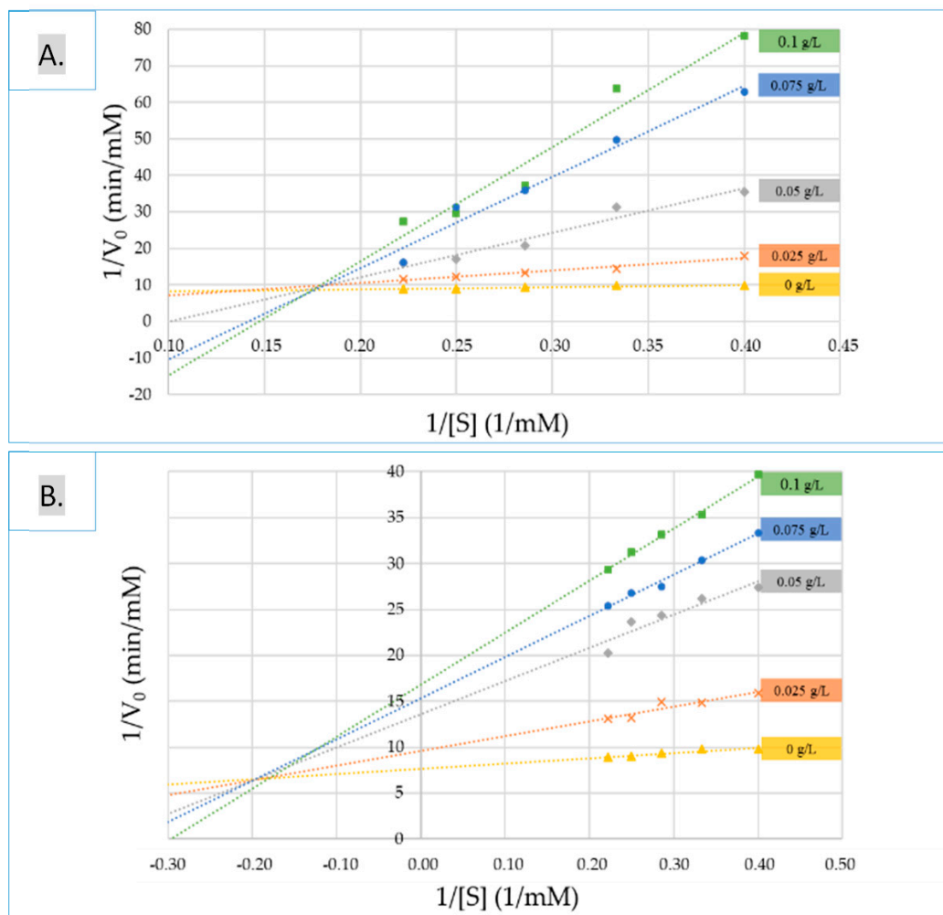
Figure 3. Lineweaver-Burk double reciprocal plots of (A) skin and (B) seed extracts at the first stage of ripening for the \alpha -glucosidase activity mode.
