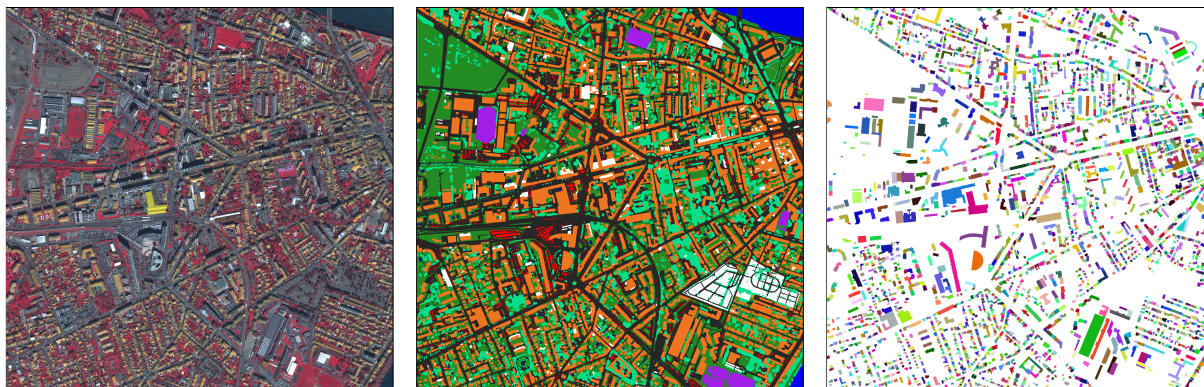
Figure 1. 1 out of 16 tiles of the SemCity Toulouse data set (876 px \times 863 px, area covered \approx 3 km 2 ). Illustrated are the satellite image (near infrared-green-blue), semantic segmentation annotation, and building instance annotation (from left to right).
