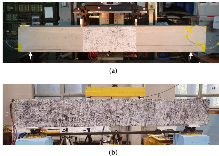
Figure 5. Front view of the beams and contract points position (a) At BAM and (b) at NEOSTRIN.
