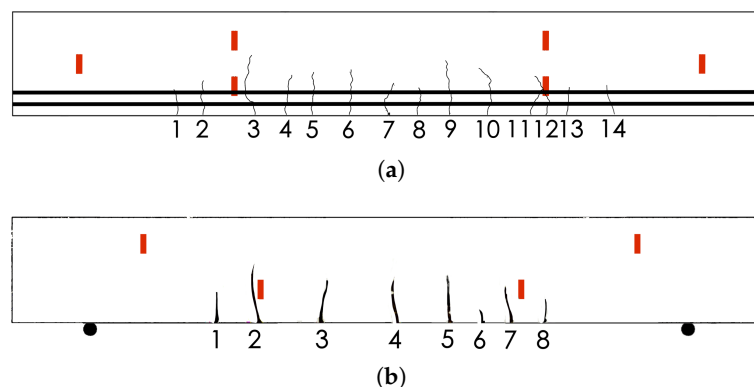
Figure 9. Cracks map of beam at (a) BAM and at (b) NEOSTRIN.
