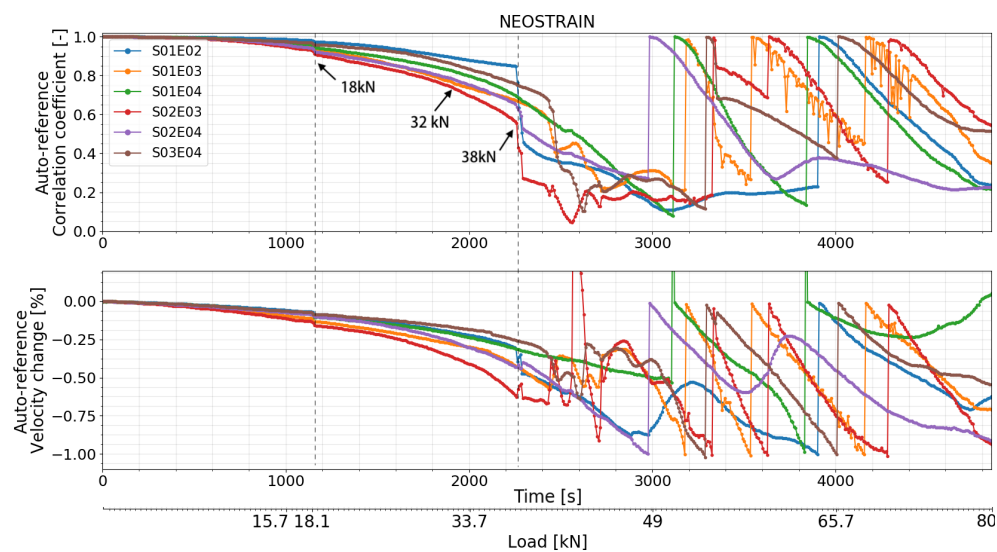
Figure 19. Correlation coefficient and relative velocity change of all the transducers combinations in test at NEOSTRIN calculated by auto reference CWI.
