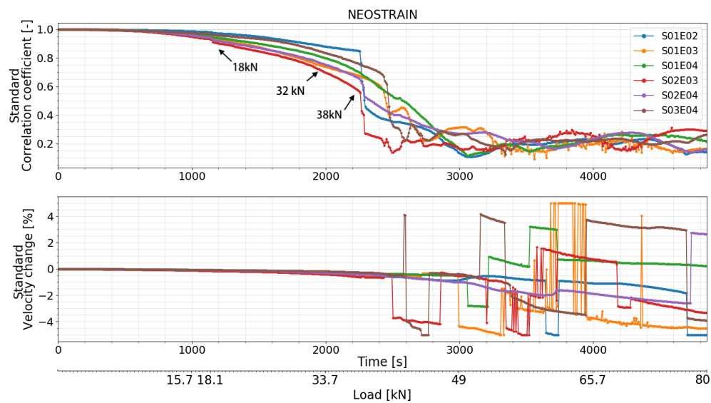
Figure 18. Correlation coefficient and relative velocity change of all the transducers combinations in test at NEOSTRIN calculated by standard CWI.
