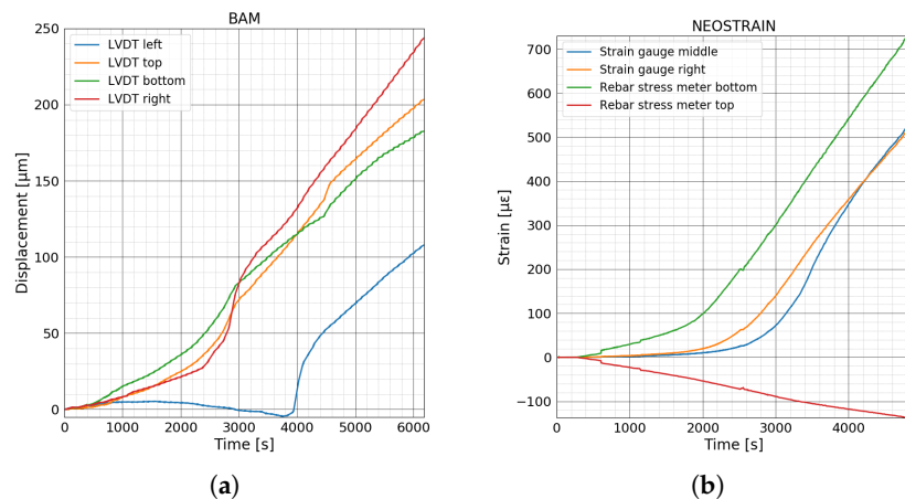
Figure 12. (a) Displacements measured by LVDT sensors at BAM. (b) Strain variation inside concrete and rebars measured by strain gauges and rebar stress meters at NEOSTRIN.
