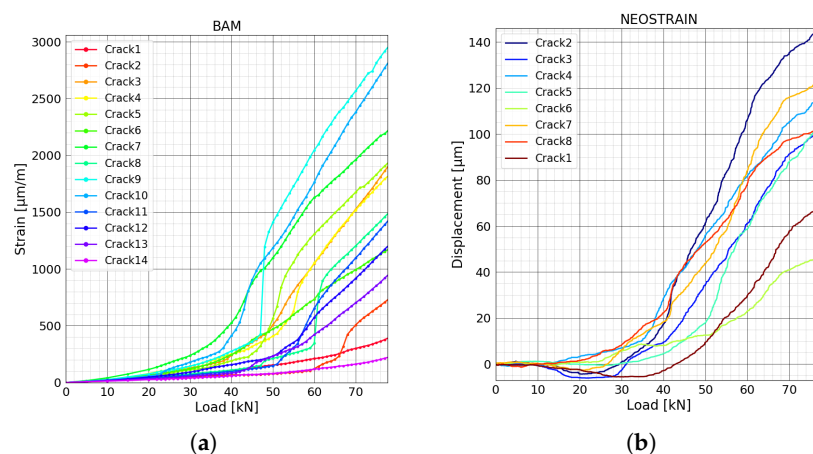
Figure 13. (a) Strain variation at position of all cracks measured by fiber line 7B at BAM. (b) Displacement at position of all cracks measured by DIC technique at NEOSTRIN.
