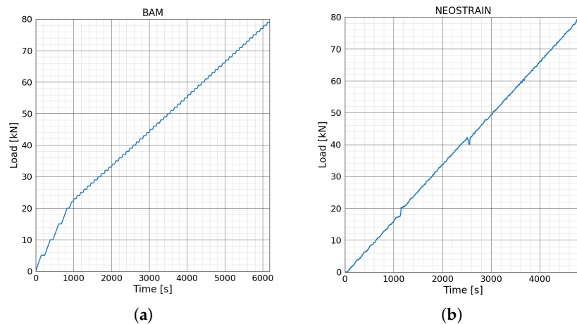
Figure 8. Loading steps of four points bending test at (a) BAM and at (b) NEOSTRIN.
