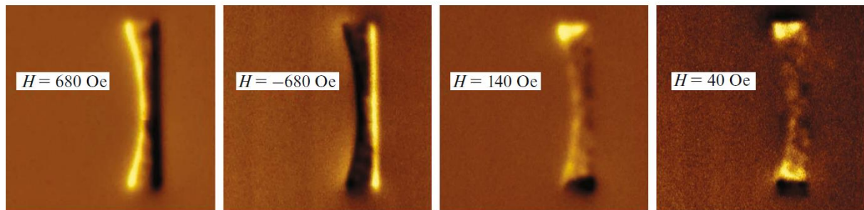
Fig. 3. Magnetic nanostrip with a parabolic profile in the presence of an external magnetic field directed in the film plane perpendicular to the long side of the structure (magnetic force microscopy; the magnetic field strength is indicated on the scans).
