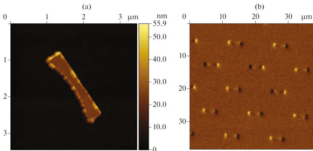
Fig. 2. (a) Topography of a magnetoelastic nanostrip with a parabolic profile (atomic force microscopy) and (b) an array of such nanostrips on a piezoelectric substrate (magnetic force microscopy).
