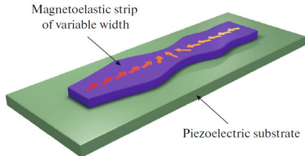
Fig. 1. Model of the domain structure in a magnetoelastic nanostrip with variable width.
