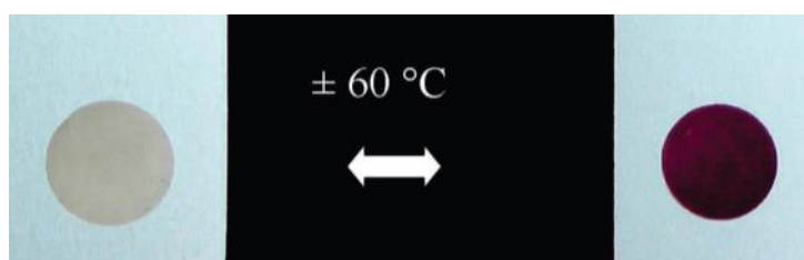
Figure 26. Thermochromic effect of the liquid crystal film [\text{Fe}(\text{C}_{12}\text{-trz})_3](4\text{-MeC}_6\text{H}_4\text{SO}_3)_2 . [119]
