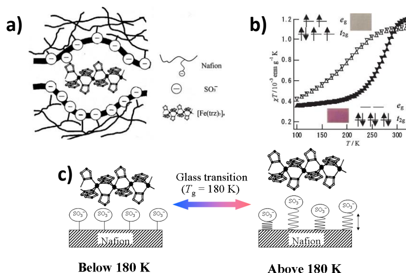
Figure 4. a) Representation of \text{Fe}^{\text{II}}(\text{Htrz})_3\text{-Nafion} complex; b) thermal variation of \chi T for \text{Fe}^{\text{II}}(\text{NH}_2\text{trz})_3\text{-Nafion} ( \diamond ) and \text{Fe}^{\text{II}}(\text{Htrz})_3\text{-Nafion} ( \bullet ); c) representation of \text{Fe}^{\text{II}}(\text{Htrz})_3\text{-Nafion} before and after the glass transition.[30,32,34]
