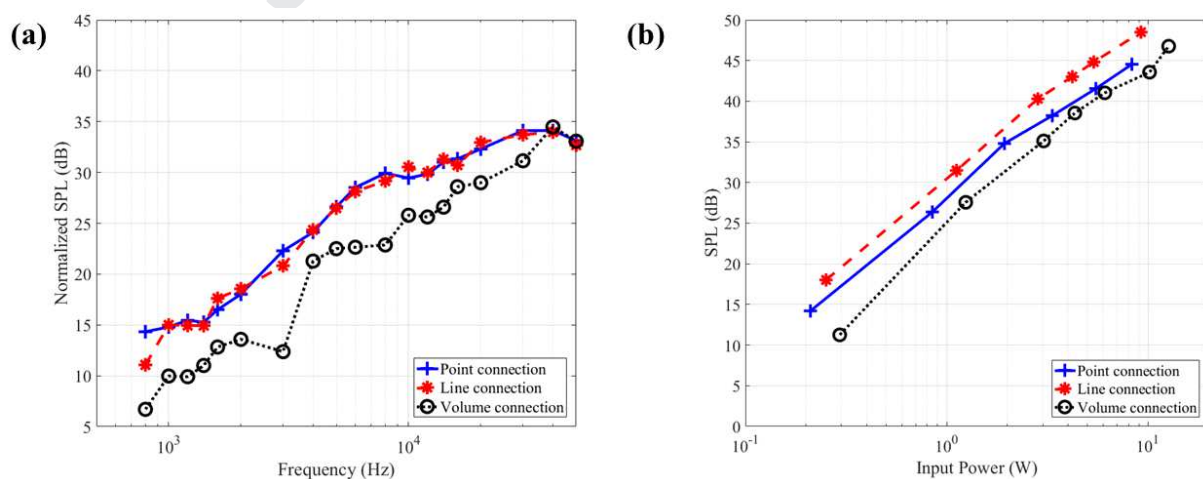
Fig. 5. (a) Acoustical frequency and, (b) power spectrum of samples of the same size but with different silver paste connections, see Table B.1.
