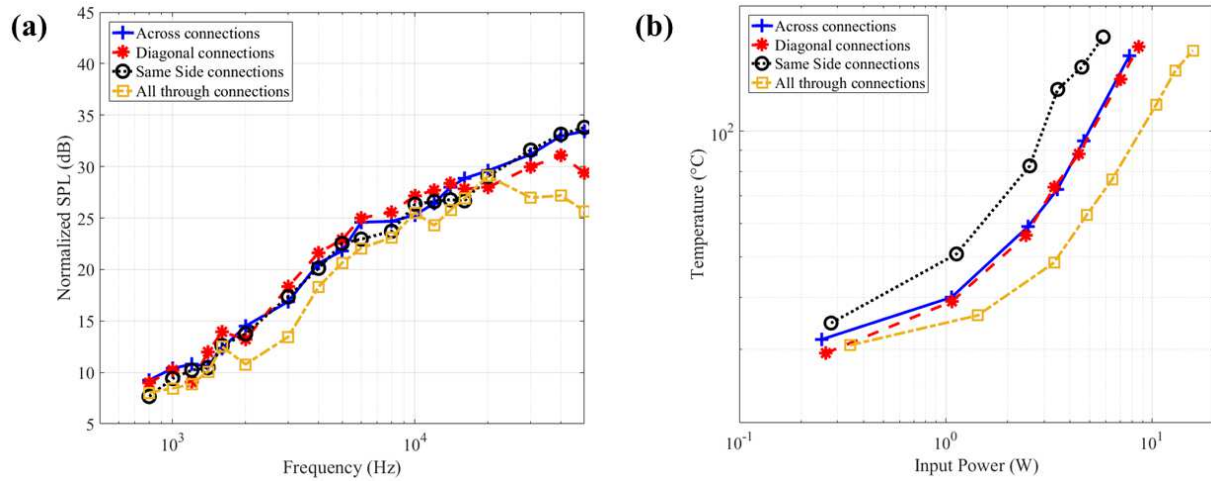
Fig. 8. (a) Acoustical frequency spectrum and (b) temperature variations of one sample with different electrical connection paths.
