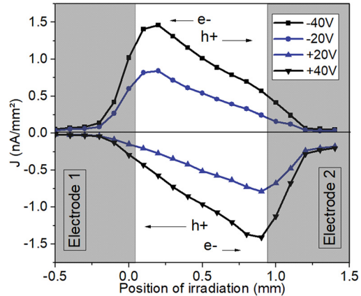
FIG. 5. Photocurrent density as a function of the position of the irradiation.
