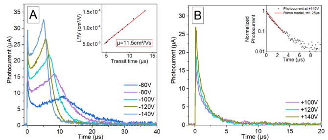
FIG. 3. (a) ToF hole photocurrent of a MAPbBr3 sample (inset: mobility calculation). (b) ToF electron photocurrent of a MAPbBr3 sample (inset: photocurrent at +140 \text{ V} and Ramo model for \tau_e = 1.25 \mu\text{s} ).
