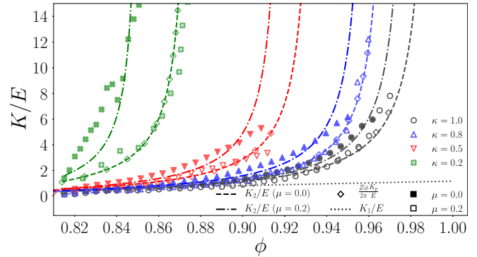
FIG. 7. Bulk modulus K normalized by E along with the micromechanical relation proposed on Eq. (10) (diamond symbols) for all values of \kappa and \mu_s = 0 . The prediction given by Eq. (13) is shown in dashed line for \mu_s = 0 and \mu_s = 0.2 and the one given by Eq. (8) is displayed in dotted line.
