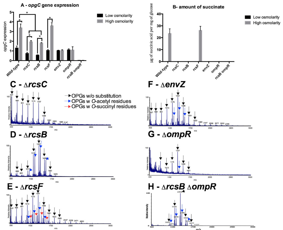
Figure 3. opgC expression level, amount of succinyl residues on purified OPGs and mass spectra of purified OPGs in the wild-type, rcsC , rcsB , rcsF , envZ , ompR and rcsB ompR mutants. (A) For the expression of the opgC::uidA gene, bacteria were grown to the mid-log phase and lysed by sonication. \beta -glucuronidase activity was measured with PNPu as a substrate. Specific activity was expressed as the change in OD405 per minute and per milligram of protein. Results are the average of three independent experiments. (B) For the quantification of the amount of succinyl residues, bacteria were grown overnight and OPGs extracted. Succinic acid content was determined with a succinic acid kit. (C–H) MALDI mass spectra acquired in positive ion mode on purified OPGs on various mutants.
