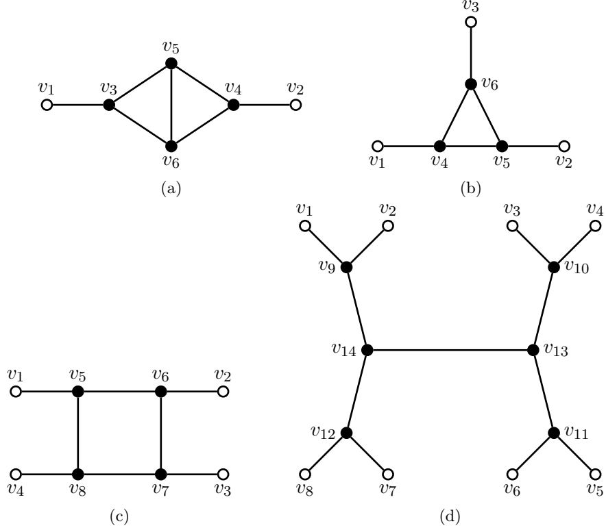
Figure 5: Configurations reduced for proving Theorem 1.14. Black vertices are vertices having their whole neighborhood being part of the configuration. White vertices may have neighbors not depicted in the configuration.
