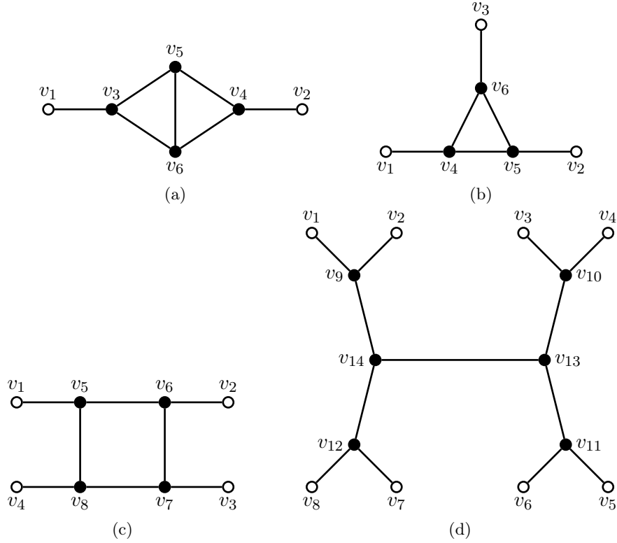
Figure 5: Configurations reduced for proving Theorem 1.13. Black vertices are vertices having their whole neighborhood being part of the configuration. White vertices may have neighbors not depicted in the configuration.
