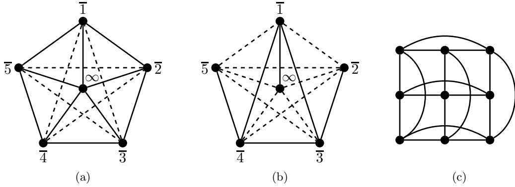
Figure 1: The signed graph (SP_5^+, \square^+) (a), the signed graph (SP_5^+, \square^+) obtained by switching the vertices \infty and \bar{1} of (SP_5^+, \square^+) (b), and the signed graph (SP_3, \square) (c). In (a), (b) and (c), solid edges are positive edges. In (a) and (b), dashed edges are negative edges. In (c), non-edges are negative edges.
