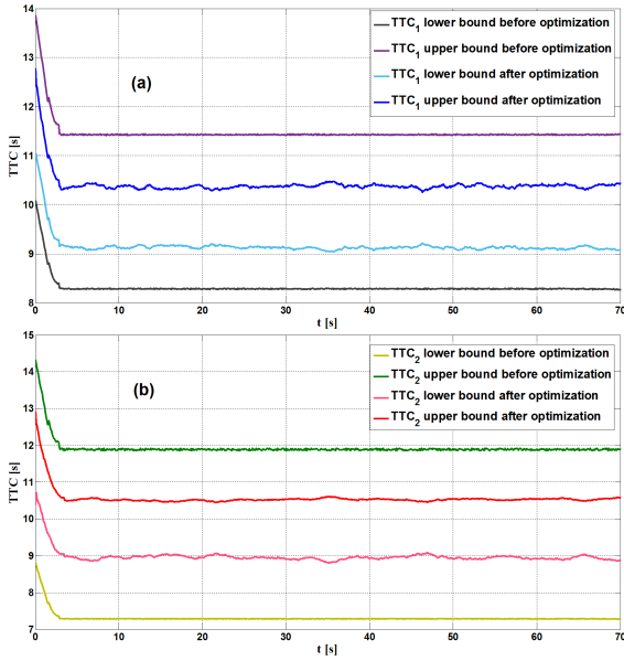
Figure 4: TTC_1 and TTC_2 enclosures with/without optimization step
