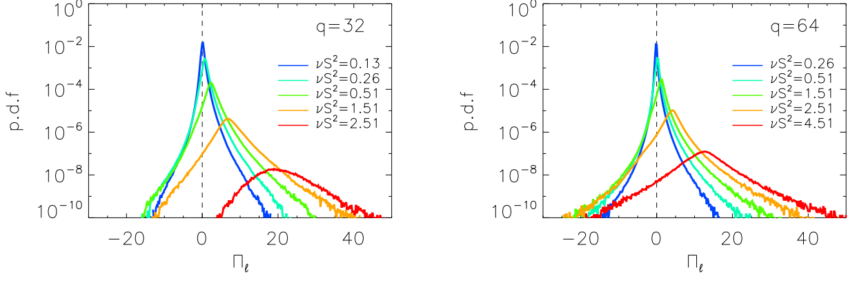
FIG. 7: The pdf of the flux conditioned on different values of the strain S_\ell for q = 32 (left) and q = 64 (right).
