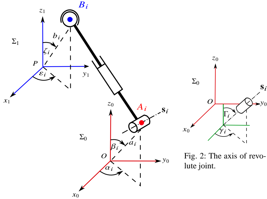
Fig. 1: Coordinates and Design Parameters of RPS Leg.
