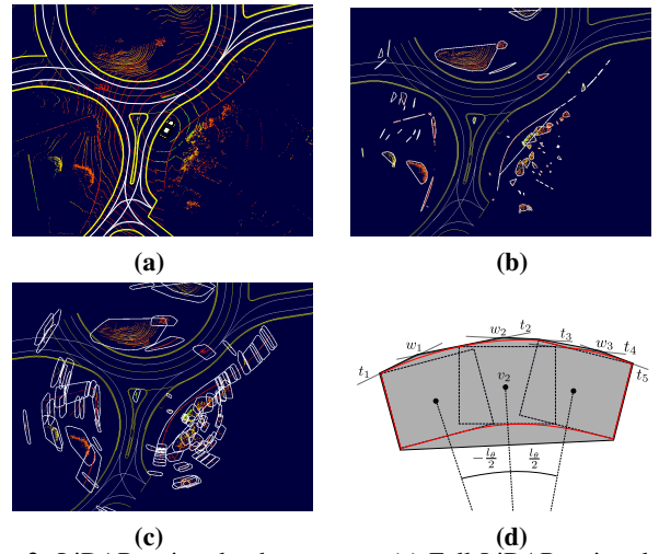
Fig. 2: LiDAR point cloud processes. (a) Full LiDAR point cloud and HD map (in yellow). (b) Clustering and bounding convex hulls computation on not-ground point cloud obtained by segmentation. (c) Convex hulls extension by localization uncertainty propagation. (d) The real occupied space obtained by the rectangle rotation is in red. The convex approximation adopted in the explained methodology is in grey.
