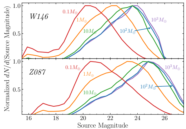
Figure 11. Low-mass lens will have much brighter source stars. Here we show the source magnitude distributions normalized to their peaks. The higher mass lenses ( \gtrsim 10 M_\oplus ) will have nearly identical distributions, but lower masses than that will strongly deviate. Upper: Source magnitude distribution in W146 . Lower: Source magnitude distribution in Z087 .
