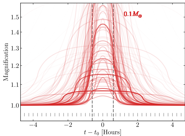
Figure 4. The rightmost panel of Figure 3, but rescaled to highlight the finer detail of light curves arising from \sim 0.1 M_{\oplus} lenses. Note that the magnification remains in log-scale, but the horizontal axis has been converted from days to hours. The vertical dashed lines are the weighted average t_E , which indicate that the Einstein timescales are generally much shorter than the observed timescales, which are set by the crossing time of the source when \rho \gg 1 . The gray vertical dashes match the 15 min observing cadence of the W146 band.
