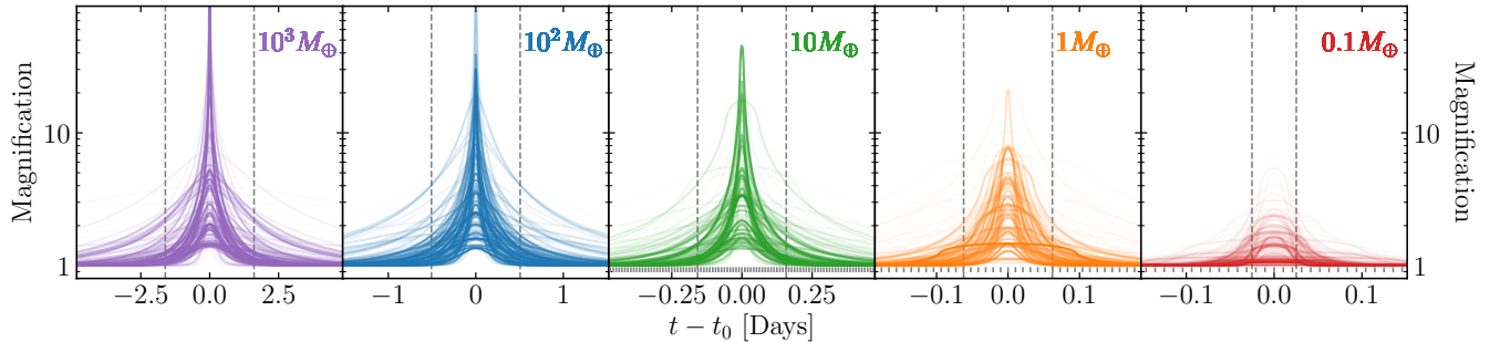
Figure 3. Samples of simulated magnification curves from events detectable by Roman at each mass of 10^3 , 10^2 , 10 , 1 , 0.1M_{\oplus} , from left to right. For each mass, we randomly select 100 events that passed our detection criteria and plot their magnification curves. The weighted average \pm t_E is indicated by the vertical dashed lines in each panel. Note the horizontal axis scale changes as mass decreases and the vertical axis uses a logarithmic scale. The black, horizontal tick marks below the curves indicate the W146 cadence; we note that they are only shown for masses of 10 M_{\oplus} and below. The transparency of each curve is proportional to the weight of the event normalized to the maximum weight of events included in the panel. In this way, darker lines exemplify events that will contribute more to the event rate for that mass bin.
