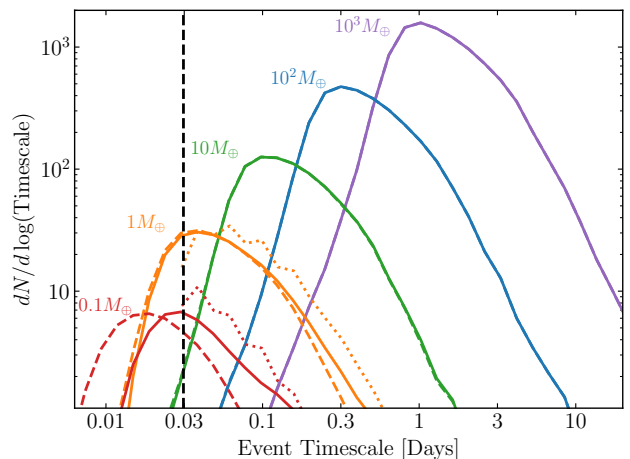
Figure 5. The distribution of detected events as a function of timescale for different lens mass populations. We plot the distributions as a function of t_E as dashed lines. The solid lines are the distributions as a function of the maximum of t_E or the source half-chord crossing time, 0.5t_c . These distributions are nearly identical for masses above 10M_{\oplus} because for these masses typically t_E \gg 0.5t_c , whereas for lower masses the timescale is largely set by the source chord crossing time. For the two lowest masses, we also plot as dotted lines for the distribution of \frac{1}{2}n_{3\sigma} \times 15\text{min} . The vertical dashed line indicates 3 \times the W146 band cadence. The cut we impose on n_{3\sigma} (e.g., the dashed vertical line) eliminates events that are formally ‘significant’ according to the \Delta\chi^2 criterion, but would likely be poorly characterized due to the small number of significant points. Interestingly, as a result of the fact that the effective event timescale saturates at the source chord crossing time for low-mass lenses, many events pass our cuts that would not in the absence of finite-source effects.
