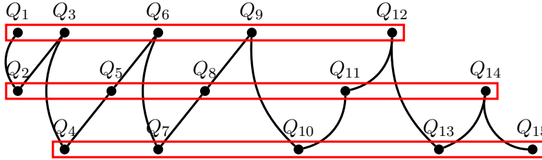
Figure 7: A neutral connector following Construction 5 where \lambda = 5 .
