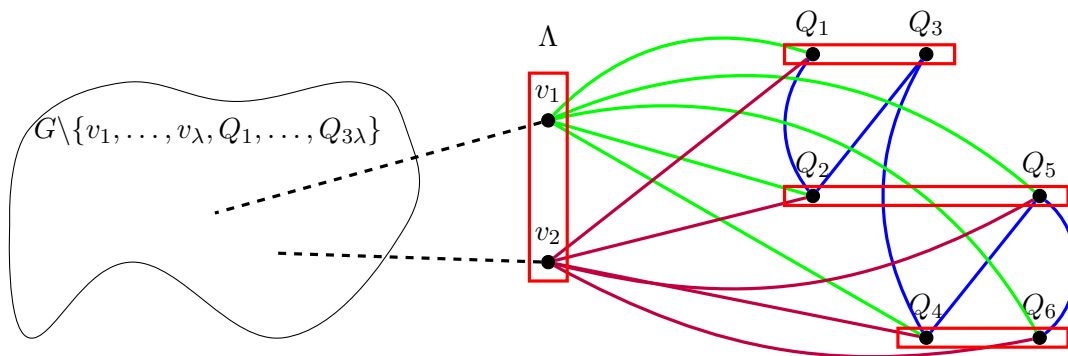
Figure 8: A graph following Construction 6 where \lambda = 2 .
