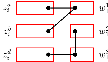
Figure 5: Illustration of Construction 3 only for a triplet c_i of the instance (\mathcal{X}, \mathcal{C}) of RX3C .
