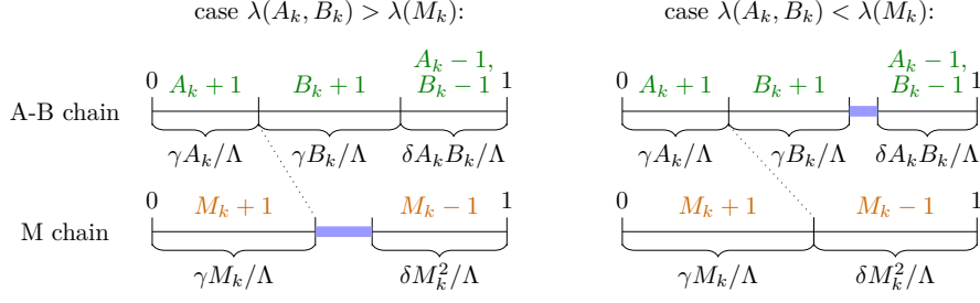
■ Figure 2 Continuous-time coupling of the A-B chain and the single-species birth-death M-chain, given that A_k \leq B_k , with \Lambda = \Lambda(A_k, B_k, M_k) . The intervals for the cases of \xi_{k+1} and their effect on the A-B chain and the M-chain are shown in green and orange, respectively. Cases that lead to stuttering steps are shown in blue. The dotted relation between intervals is proven in Lemma 4.
