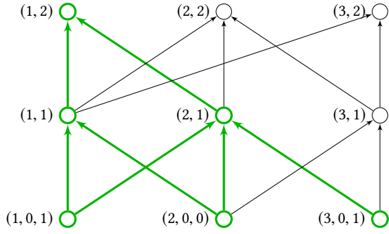
Figure 2: Example of a process-time graph PT^2 at time t = 2 with n = 3 processes and initial values x = (1, 0, 1) . Process 1's view V_{\{1\}}(PT^2) is highlighted in bold green.
