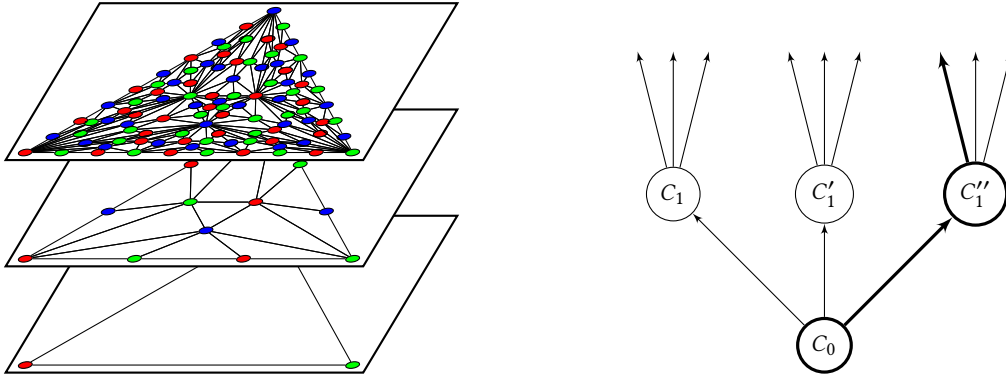
Figure 1: Comparison of the combinatorial topology approach and the point-set topology approach: The combinatorial topology approach (left) studies sequences of increasingly refined spaces in which the objects of interest are simplices (corresponding to configurations). The point-set topology approach (right) studies a single space in which the objects of interest are executions (i.e., infinite sequences of configurations).
