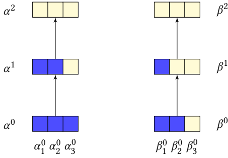
Figure 3: Comparison of the P -view, minimum, and common prefix topologies. The first three configurations of each of the two executions \alpha and \beta with three processes and two different possible local states (dark blue and light yellow) are depicted. We have d_{\max}(\alpha, \beta) = d_{\{3\}}(\alpha, \beta) = 1 , d_{\{2\}}(\alpha, \beta) = 1/2 , and d_{\min}(\alpha, \beta) = d_{\{1\}}(\alpha, \beta) = 1/4 .
