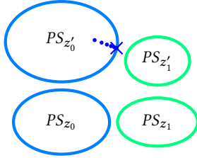
Figure 4: Examples of two connected components of the decision sets PS(0) = PS_{z_0} \cup PS_{z'_0} and PS(1) = PS_{z_1} \cup PS_{z'_1} for a compact message adversary. They are closed in \mathcal{PT}^\omega , hence contain all their limit points (marked by \times ) and have a distance > 0 by Theorem 5.13.
