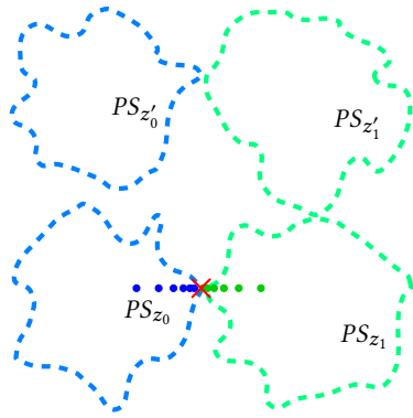
Figure 5: Examples of two connected components of the decision sets PS(0) = PS_{z_0} \cup PS_{z'_0} and PS(1) = PS_{z_1} \cup PS_{z'_1} for a non-compact message adversary. They are not closed in \mathcal{PT}^\omega and may have distance 0; common limit points (like for PS_{z_0} and PS_{z_1} , marked by \times ) must hence be excluded by Corollary 5.18.
