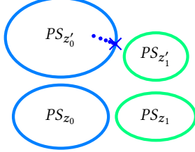
Figure 4: Examples of two connected components of the decision sets PS(0) = PS_{z_0} \cup PS_{z'_0} and PS(1) = PS_{z_1} \cup PS_{z'_1} for a compact message adversary. They are closed in \mathcal{PT}^\omega , hence contain all their limit points (marked by \times ) and have a distance > 0 by Theorem 5.13.
