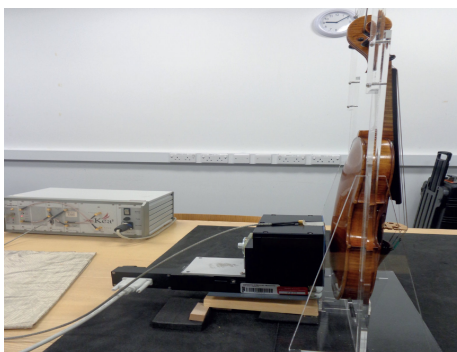
Figure: Portable NMR at the Ashmolean Museum, Oxford
