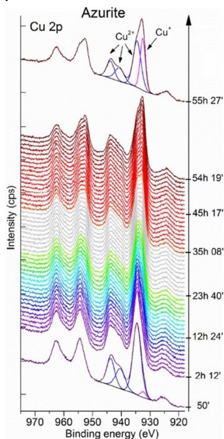
Figure: Evolution of Cu 2p XPS of azurite pigment at different time intervals during soft X-ray exposure. Curve fitting of Cu 2p_{3/2} displays the increase of \text{Cu}^+ versus \text{Cu}^{2+} after X-ray irradiation.
