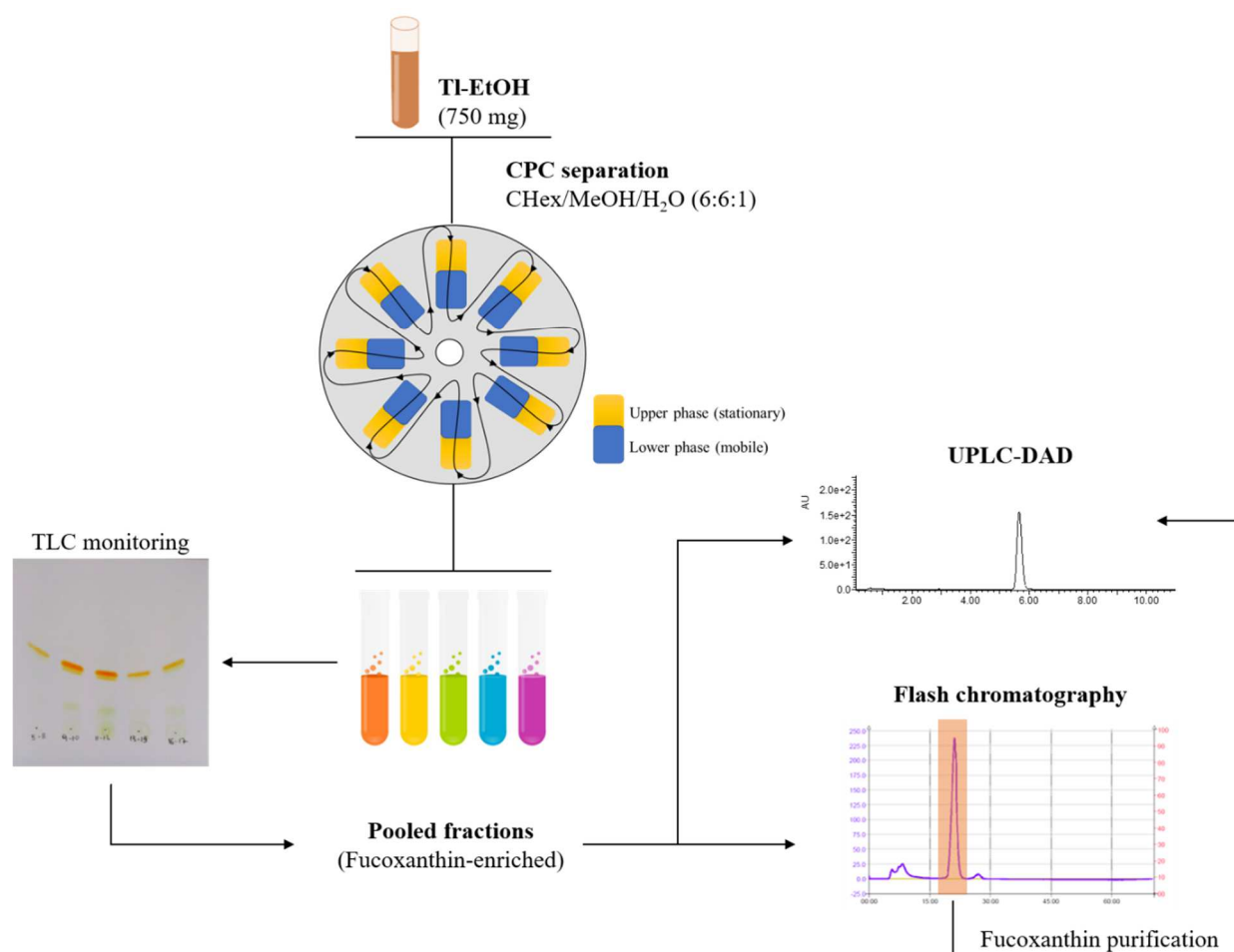
Fig. 5. Flowchart of the CPC-concentration and flash chromatography purification of fucoxanthin from T. lutea ethanol extract (TI-EtOH). CPC fractions were monitored by TLC and UPLC-DAD, final yield and purity were determined by UPLC-DAD.
