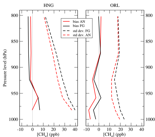
Fig. 11. Vertical profiles of bias (solid lines) and standard deviation (std dev., dashed lines) between measured and first-guess (FG, in black) or analyzed (AN, in red) CH 4 concentrations (ppbv) at ORL and HNG locations in 2004. Positive values for the bias indicate that the simulated concentrations are higher than the measurements.
