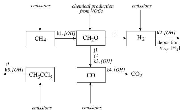
Fig. 1. Schematic of the simplified chemistry mechanism SACS: j_1 – j_3 and k_1 – k_5 are the constants of the reactions or of ensembles of reactions. [OH] and the variables indicated in italics are directly optimized by the data assimilation system.
