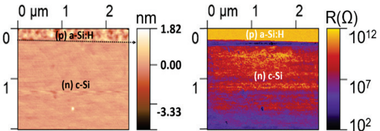
Figure 2. C-AFM image illustrating a cleaved section of a (p) a-Si:H/(n) c-Si heterointerface. Left : topography; right : local resistance mapping (logarithmic scale). Data from Ref.[30].
