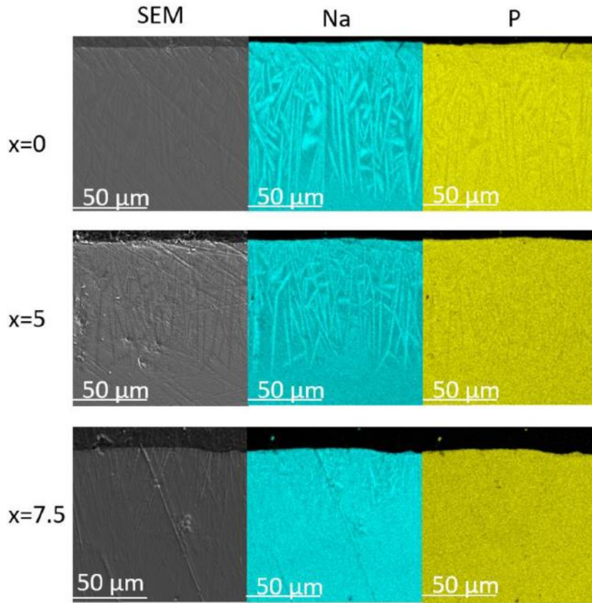
Fig. 4. Elemental mapping of the crystals in the glasses' SEM images after heat treatment A.
