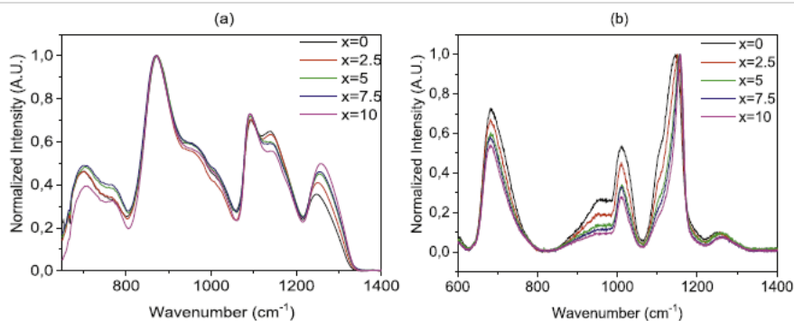
Fig. 1. IR (a) and Raman (b) spectra of the investigated glasses.
