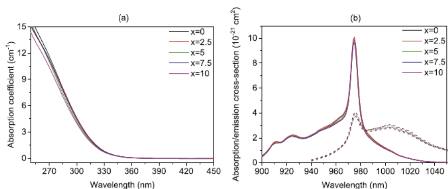
Fig. 2. Absorption spectra (a) and absorption/emission (solid/dashed) cross sections centered at 975 nm (b) of the investigated glasses.
