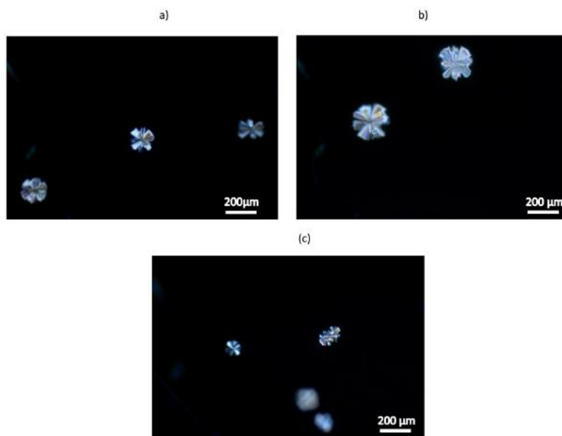
Fig. 9. Optical images of the crystals found in the heat treated glasses with x = 0 after HT-A (a), HT-C (b) and HT-D (c). The images were taken with 5x microscope magnification in transmission mode using cross-polarized configuration of the microscope.
