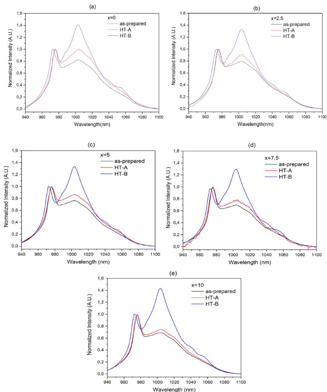
Fig. 6. Normalized emission spectra of the glasses with (a) x = 0 , (b) x = 2.5 , (c) x = 5 , (d) x = 7.5 and (e) x = 10 prior to and after heat treatment A or B. Excited at 900 nm.
