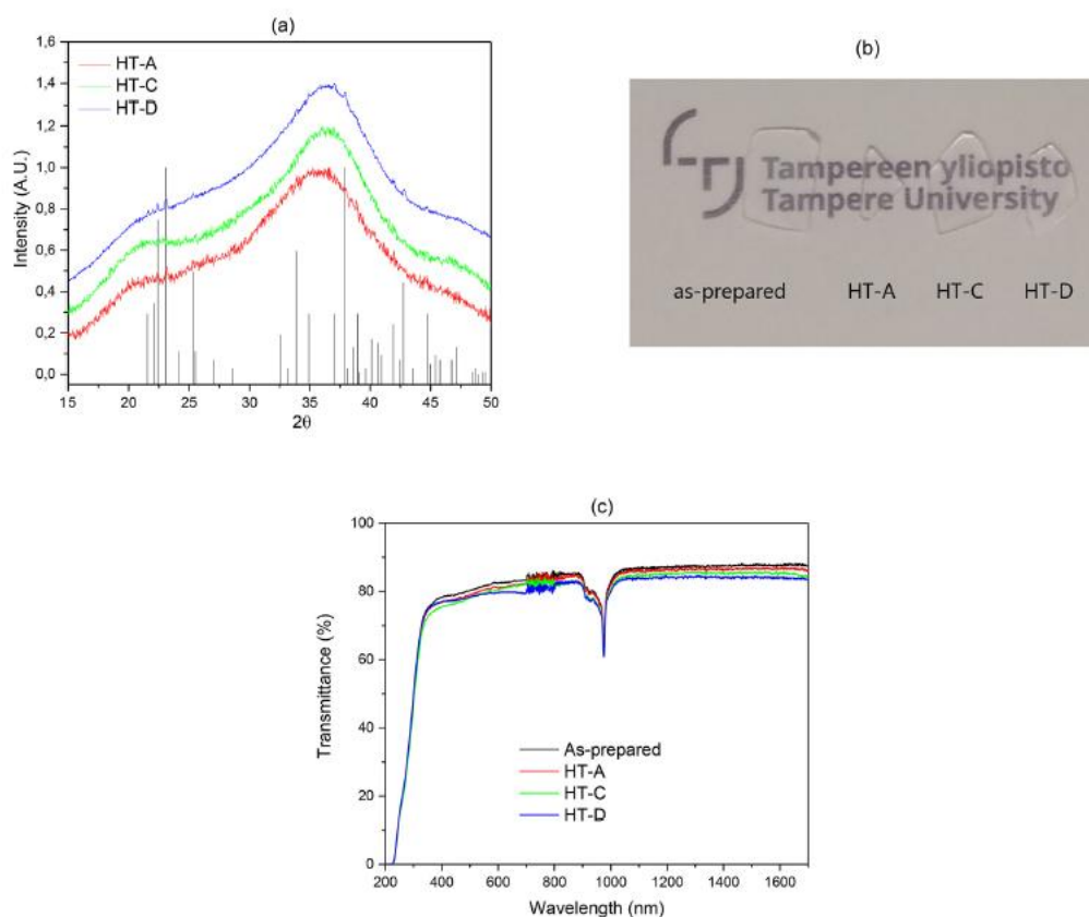
Fig. 8. XRD patterns (also shown is the XRD pattern of \text{Na}_5\text{P}_3\text{O}_{10} -I [00-010-0179]) (a), the pictures (b) and the transmittance spectra (c) of heat treated glasses with x = 0 .
