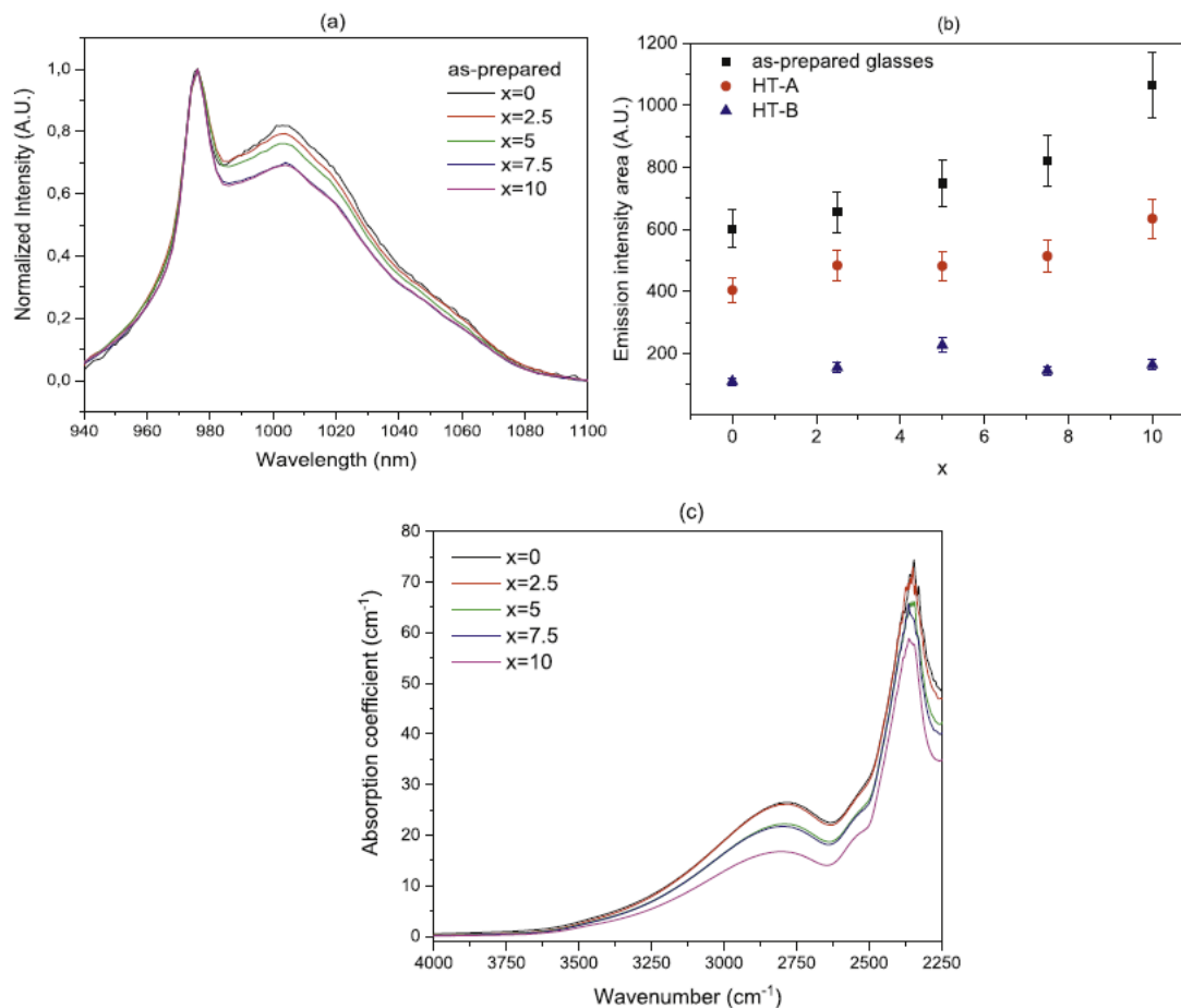
Fig. 3. Emission spectra measured using a 900 nm excitation (a), integrated area of the emission band (b) and IR absorption spectra of the glasses (c).
