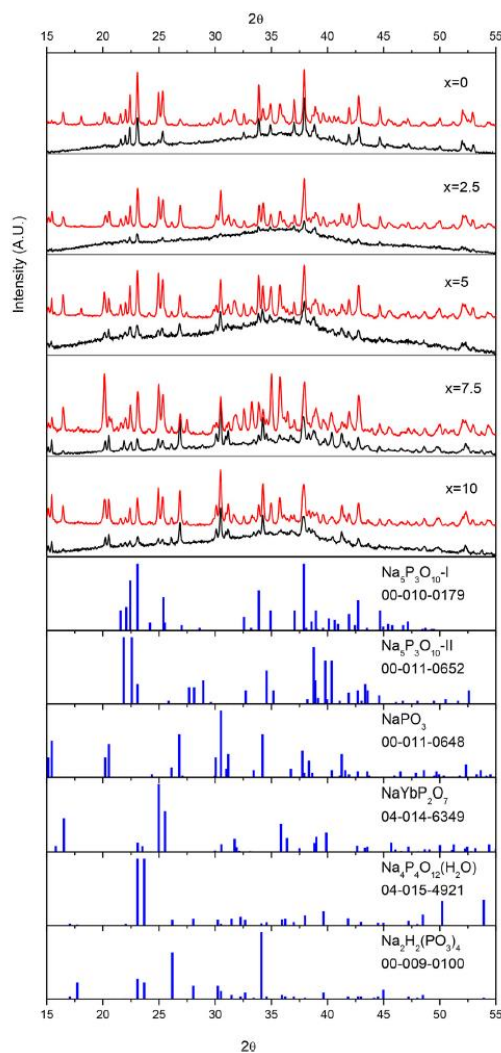
Fig. 5. XRD of the investigated glasses after heat treatment A (black), and B (red). (For interpretation of the references to colour in this figure legend, the reader is referred to the Web version of this article.)
