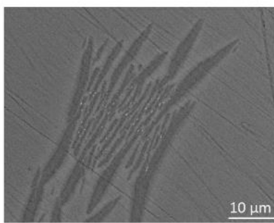
Fig. 7. SEM image of crystals found in the volume of the glass with x = 0 after heat treatment A.
