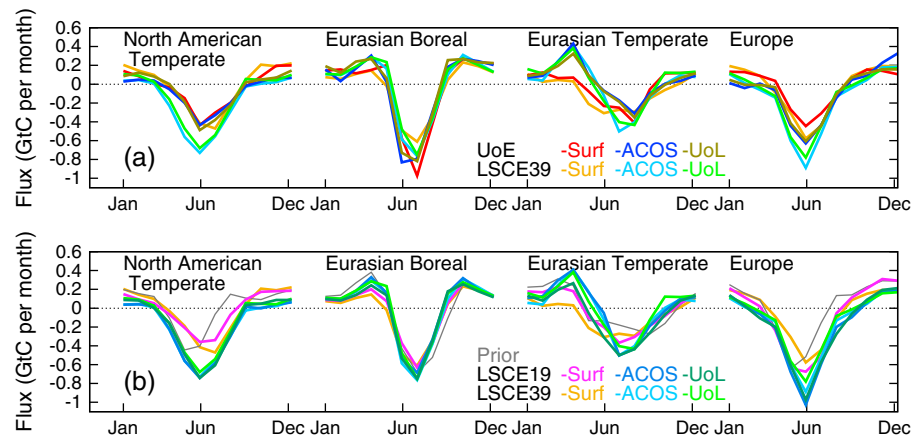
Figure 2. Regional seasonal CO 2 flux estimates in four of the regions of Figure 1. (a) Comparison of the UoE and the LSCE-39 results. (b) Comparison of the LSCE-19 results, the LSCE-39 results, and the LSCE prior fluxes. A positive flux is a flux to the atmosphere.
