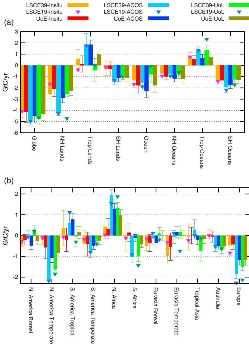
Figure 1. Large-scale annual mean natural (fossil fuel removed) CO 2 budgets of the nine atmospheric inversions from the UoE, LSCE-39, and LSCE-19 inversion systems, with in situ data and two GOSAT products (ACOS and UoL) for 2010 with their respective 1 sigma uncertainty (except for LSCE-19). NH (SH) corresponds to latitudes north (south) of 20°N (20°S). A positive flux is a flux to the atmosphere.
