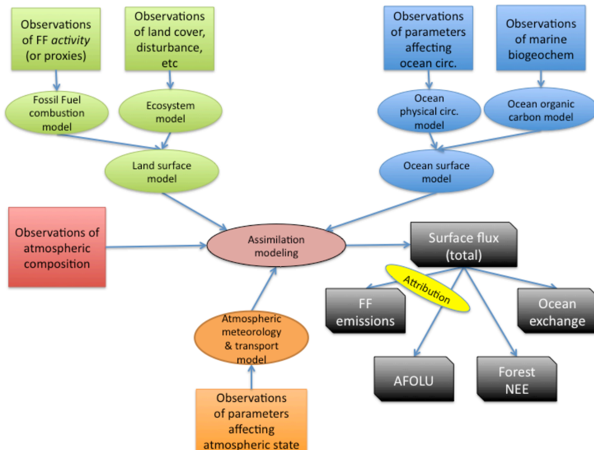
Figure 9. Conceptual illustration of a global carbon-cycle data assimilation system relying on operational carbon-cycle flux and pool measurements.
