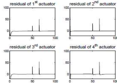
Fig. 6. Residuals r_i for to the detection and identification bank
