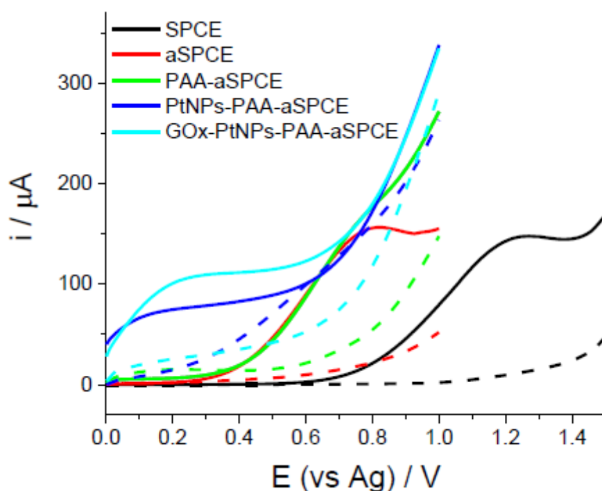
Figure 3. Anodic linear scan voltammetry responses of the different electrode modification steps in the absence (dashed lines) and the presence of 5M of H_2O_2 (solid lines) in 0.1 M phosphate buffer solution. SPCE: Screen-printed carbon electrodes, aSPCE: activated SPCE, PAA: Poly(Azur A), PtNPs: Platinum Nanoparticles, GOx: glucose oxidase. Reproduced with permission of [108], Copyright 2020, MDPI.
