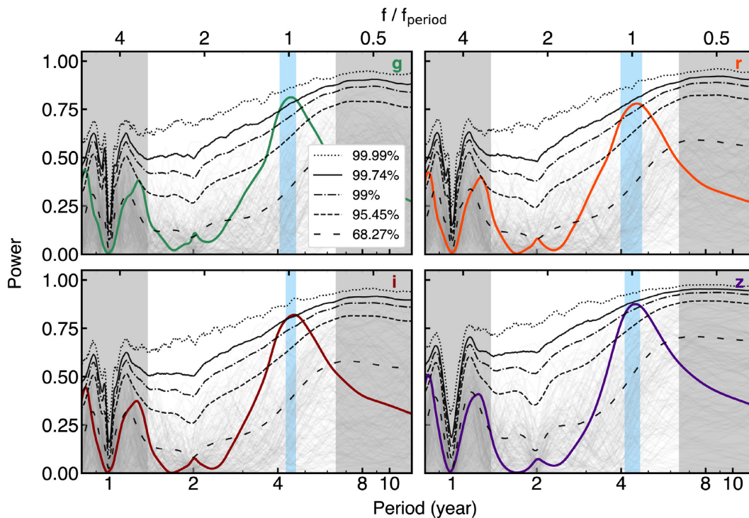
Figure 4. Generalized Lomb-Scargle periodogram showing the periodicity detection of J0252. A periodicity (see P_{\text{GLS}} in Table 2) is detected at 99.95 per cent, 99.43 per cent, 99.78 per cent, and 99.59 per cent single-peak significance (with global p values of 1.2 \times 10^{-3} , 5.8 \times 10^{-3} , 2.6 \times 10^{-3} , and 8.4 \times 10^{-3} accounting for the look elsewhere effect in the whole frequency range being searched; Chen et al. 2020) in the griz bands. The confidence levels are calculated from 50 000 tailored simulations assuming random, red noise variability. The grey curves show 200 examples drawn from the 50 000 for clarity. The cyan shaded region indicates the period uncertainty estimated using ranges above the >99.74 per cent significance for the gi bands and above the >99.00 per cent significance for the rz bands. The grey shaded regions mark the small time-scales (<500 d) on which a periodicity may be subject to artefacts due to seasonal gaps and low cadence, and the large time-scales (defined as total time baseline <3 cycles) where the data are more subject to false periodicity from stochastic quasar variability (Vaughan et al. 2016).
