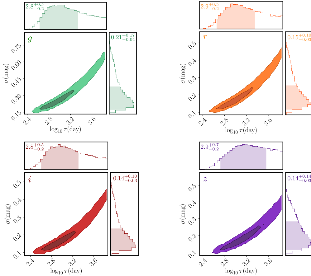
Figure 2. DRW model parameter estimates for J0252. The 2D contours show the 68 per cent and 95 per cent confidence levels estimated from the MCMC analysis. The histograms show the projected 1D probability density distributions for \sigma and \tau (observed frame). Labelled on each panel are their best-fitting value and the 1\text{-}\sigma (estimated from the 68 per cent confidence levels denoted by the shaded histograms) uncertainties. The total light-curve baseline ( \sim 7300 d) is more than 10 times larger than the correlation time-scale ( \sim 630 d in observed frame), so that the correlation time-scale recovers the true value (Kozłowski 2017).
