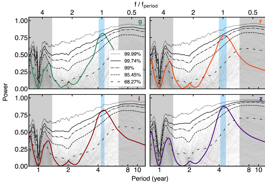
Figure 4. Generalized Lomb-Scargle periodogram showing the periodicity detection of J0252. A periodicity (see P_{\text{GLS}} in Table 2) is detected at 99.95 per cent, 99.43 per cent, 99.78 per cent, and 99.59 per cent single-peak significance (with global p values of 1.2 \times 10^{-3} , 5.8 \times 10^{-3} , 2.6 \times 10^{-3} , and 8.4 \times 10^{-3} accounting for the look elsewhere effect in the whole frequency range being searched; Chen et al. 2020) in the griz bands. The confidence levels are calculated from 50 000 tailored simulations assuming random, red noise variability. The grey curves show 200 examples drawn from the 50 000 for clarity. The cyan shaded region indicates the period uncertainty estimated using ranges above the >99.74 per cent significance for the gi bands and above the >99.00 per cent significance for the rz bands. The grey shaded regions mark the small time-scales (<500 d) on which a periodicity may be subject to artefacts due to seasonal gaps and low cadence, and the large time-scales (defined as total time baseline <3 cycles) where the data are more subject to false periodicity from stochastic quasar variability (Vaughan et al. 2016).
