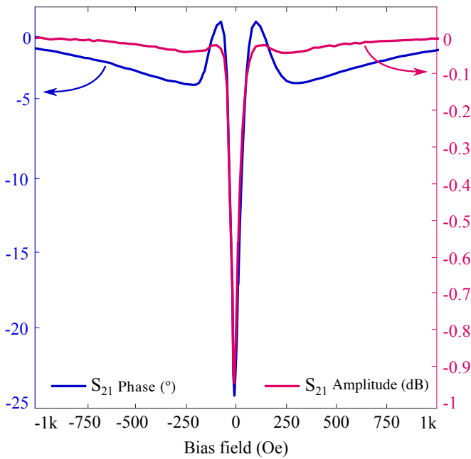
FIG. 13. Complex S_{21} response (phase in blue, magnitude in magenta) of the SAW delay line operated at 410 MHz as a function of the bias magnetic field applied along the hard axis of the multilayered TbCo 2 /FeCo nanostructured thin film.
