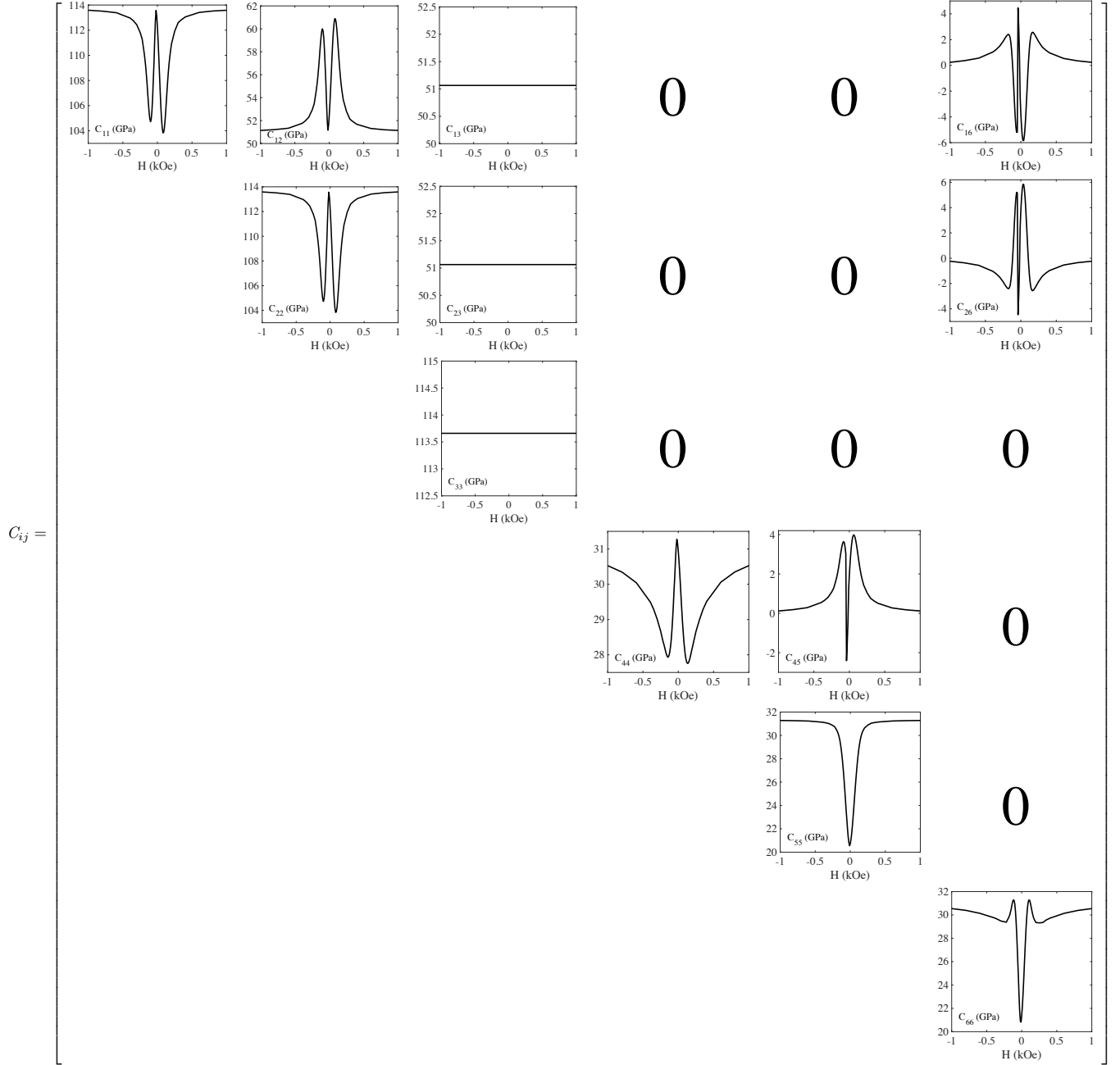
FIG. 22. Magnetic field dependency of the elastic stiffness constant tensor when a bias magnetic field is applied along the hard axis of a multilayered TbCo 2 /FeCo thin film Quartz ST-X90° cut.
