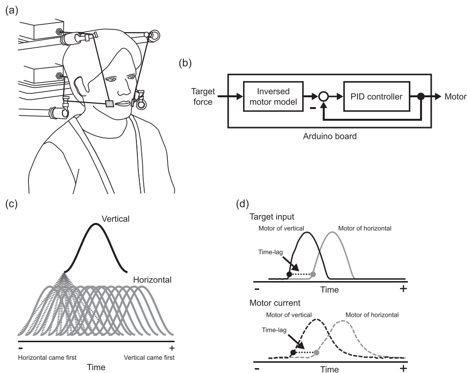
Fig. 1. (a) One example of experimental configuration using a bi-directional skin stretch perturbation system, jointly applied on the two sides of the mouth. (b) Block diagram of force control for the motor. (c) Temporal pattern of vertical and horizontal stimulation with 14 values of time-lag. (d) Schematic illustration of the calculation of the time-lag between the two motors at the target input stage (top) and at the actual motor current stage (bottom). Black and gray lines represent the time course patterns, respectively, for the vertical and the horizontal motors. Dotted line represents the time-lag between the two components. This representative example corresponds to a case where the vertical motor leads the horizontal one.
