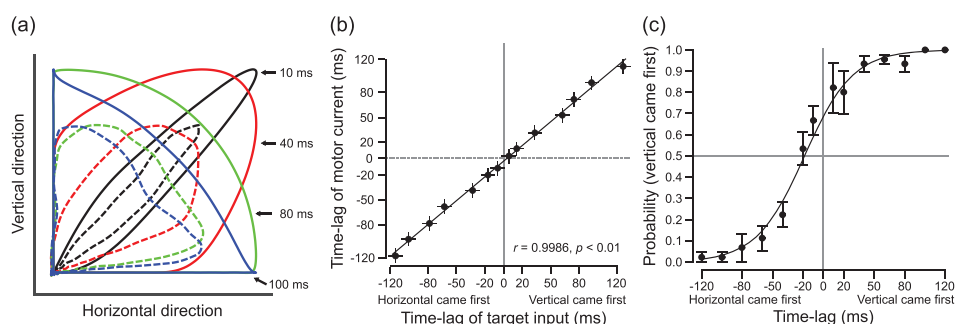
Fig. 2. (Color online) (a) Spatial trajectories resulting from the combined action of the two motors obtained in one representative trial in 10, 40, 80, and 100 ms time-lag conditions. Solid lines represent the trajectories for target input and dashed lines for motor current. Each color corresponds to each time lag condition. (b) Relationship between time-lags for target inputs and for actual motor currents, together with the corresponding regression line and correlation value. Each dot represents the value averaged across 15 trials. Error bars represent standard errors. (c) Judgement probabilities averaged over the three participants and the estimated psychometric function in the temporal order judgement test. Each dot indicates the averaged probability and error bars represent standard error across the participants.
