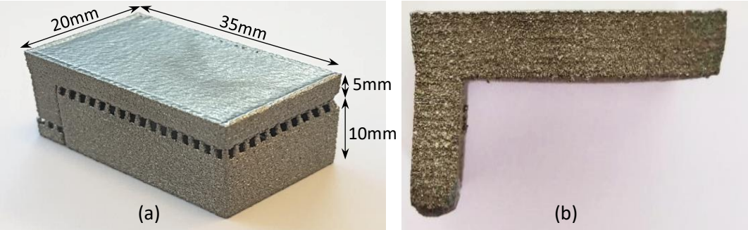
Figure 4: (a) As-fabricated part (with support) (b) Overhang part without support
