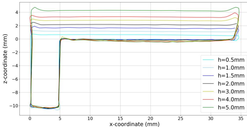
Figure 19: 2D measured profiles of parts with different overhang heights
