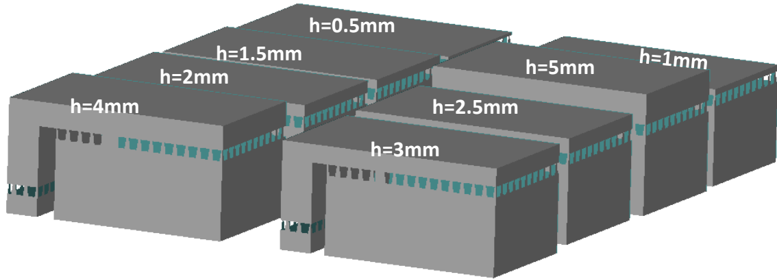
Figure 18: Manufactured parts with different overhang volume heights ( h )
