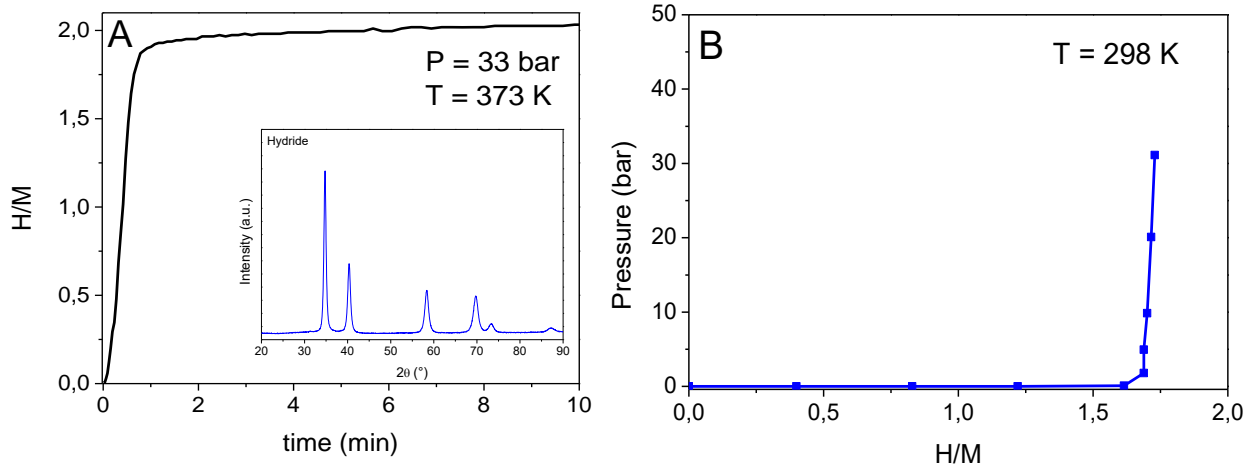
Figure 2. A: First cycle absorption kinetics for \text{Ti}_{0.30}\text{V}_{0.25}\text{Zr}_{0.10}\text{Nb}_{0.25}\text{Ta}_{0.10} at 373 K (inset: XRD of the hydride phase with \lambda_{\text{Cu K-}\alpha} = 1.5406 \text{ \AA} ). B: Pressure-Composition-Isotherm at 298 K for the second absorption cycle.
