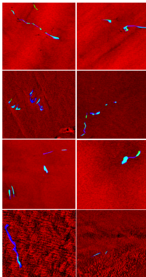
Figure 7: Example of a prediction result on Envisat SAR images from a set of tests, good predictions (light blue), false alarms (green), non-detections (dark blue).
