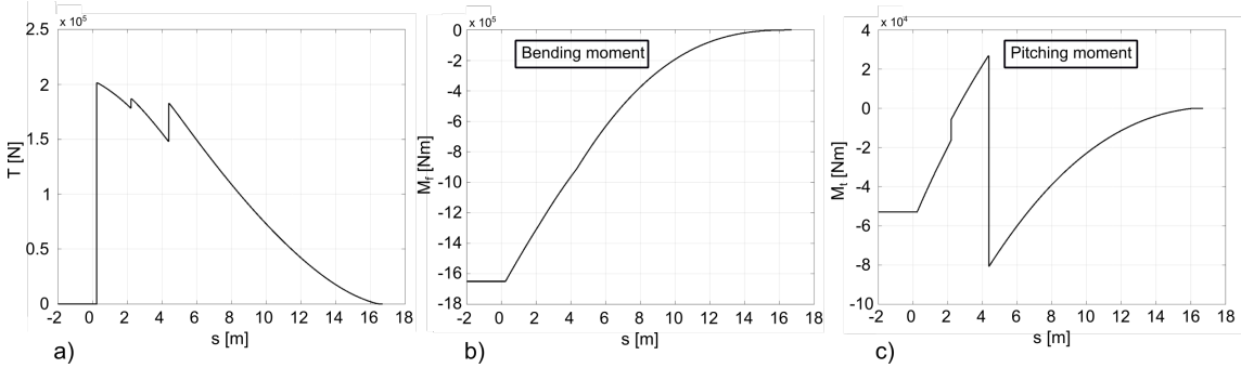
Figure 7: (a) Shear load, (b) bending moment and (c) pitching moment span-wise distribution of the inverted flight condition (LC2).
