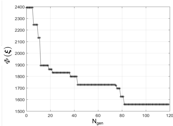
Figure 14: Evolution of the wing-box structural mass, \Phi (ξ) vs. the generation number ( N_{gen} )
