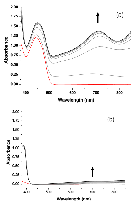
Fig. 3. UV-Visible spectra of aqueous solutions of (a) PMo 12 (0.1 mM) and FMN (0.1 mM) followed for 16 min. after addition of NADH (1 mM) and (b)
