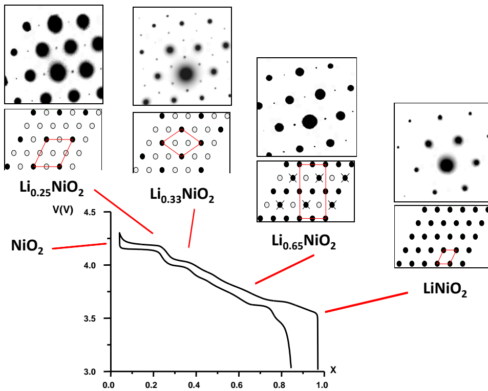
Figure 8. First cycle galvanostatic charge and discharge of a \text{Li} // \text{Li}_x\text{NiO}_2 battery. Electron diffraction and lithium/vacancy ordering for peculiar compositions.
