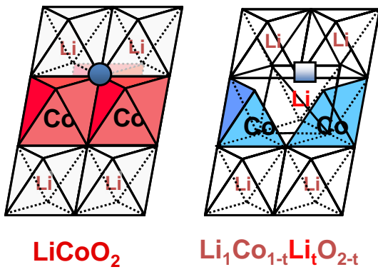
Figure 7. Effect of the presence of Li ions in the cobalt layer of \text{LiCoO}_2 phases. In the over lithiated phase two \text{IS-Co}^{3+} ions are in square pyramidal environment. Adapted with permission. Levasseur S., Ménétrier M. et al. Chem. Mater. 2003, 15, 348 Copyright 2020, ACS.
